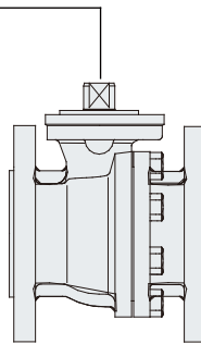
Ball valve
