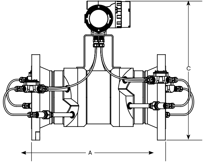
Dimensions and weights in metric units
